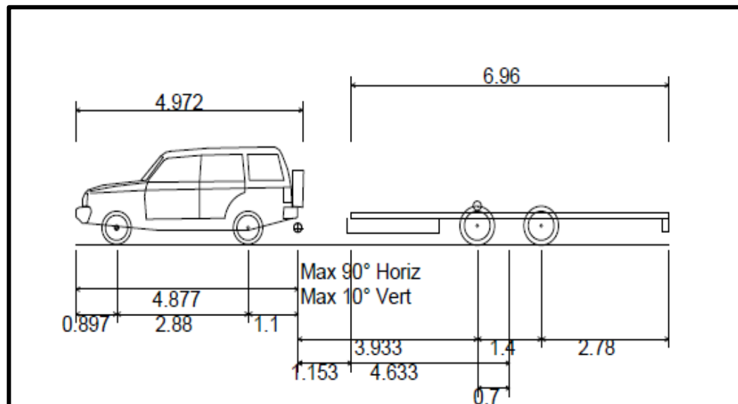
Figure 1: Dimensions of \square x with trailer
